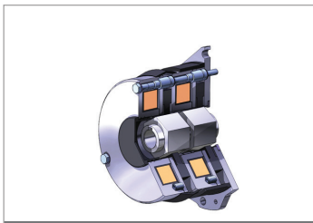
Electromagnetic Tandem Spring Applied Brake
